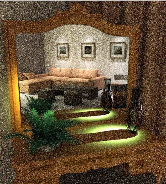
Path tracing
